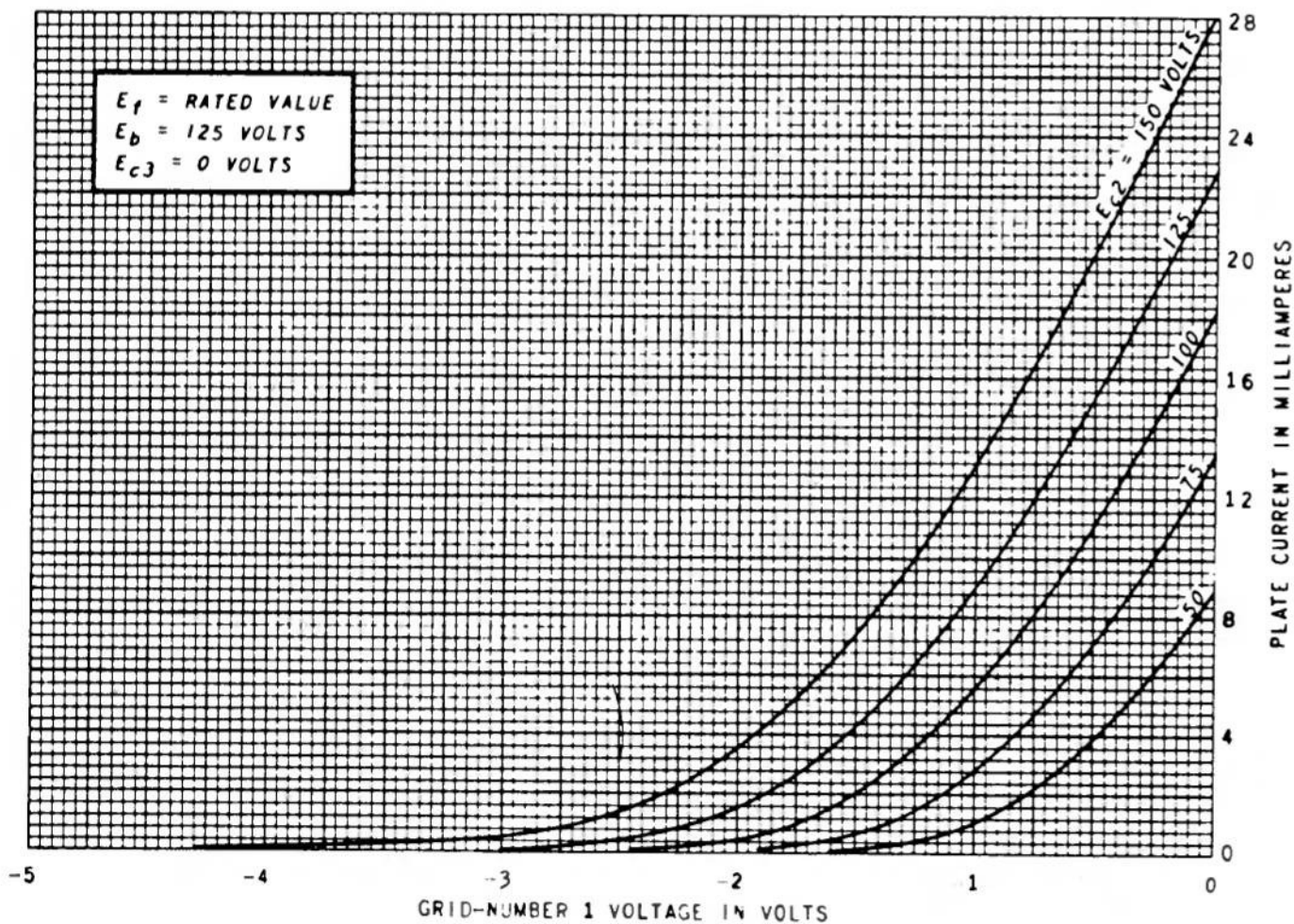
FIGURE 5, 6BN11 AVERAGE TRANSFER CHARACTERISTICS
