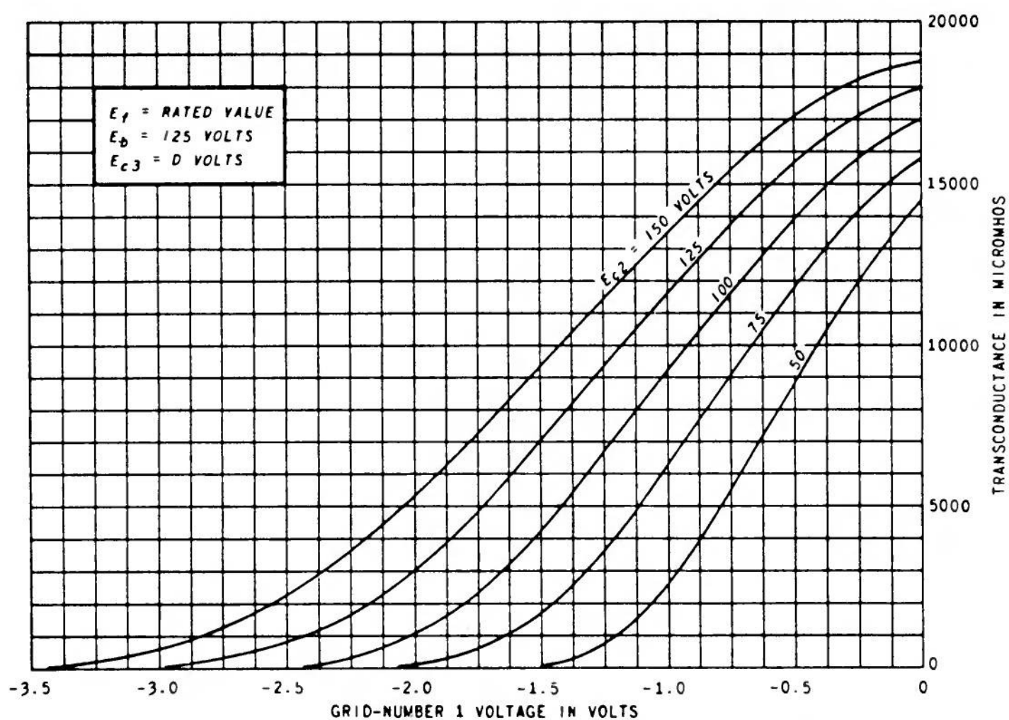
FIGURE 6, 6BN11 AVERAGE TRANSFER CHARACTERISTICS
