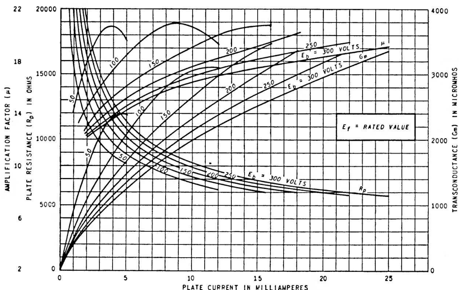
FIGURE 3, 12AU7 AVERAGE CHARACTERISTICS
