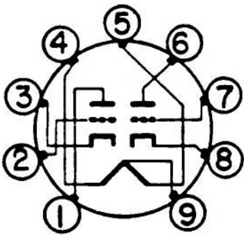
FIGURE 2, 12AU7 BASING DIAGRAM
