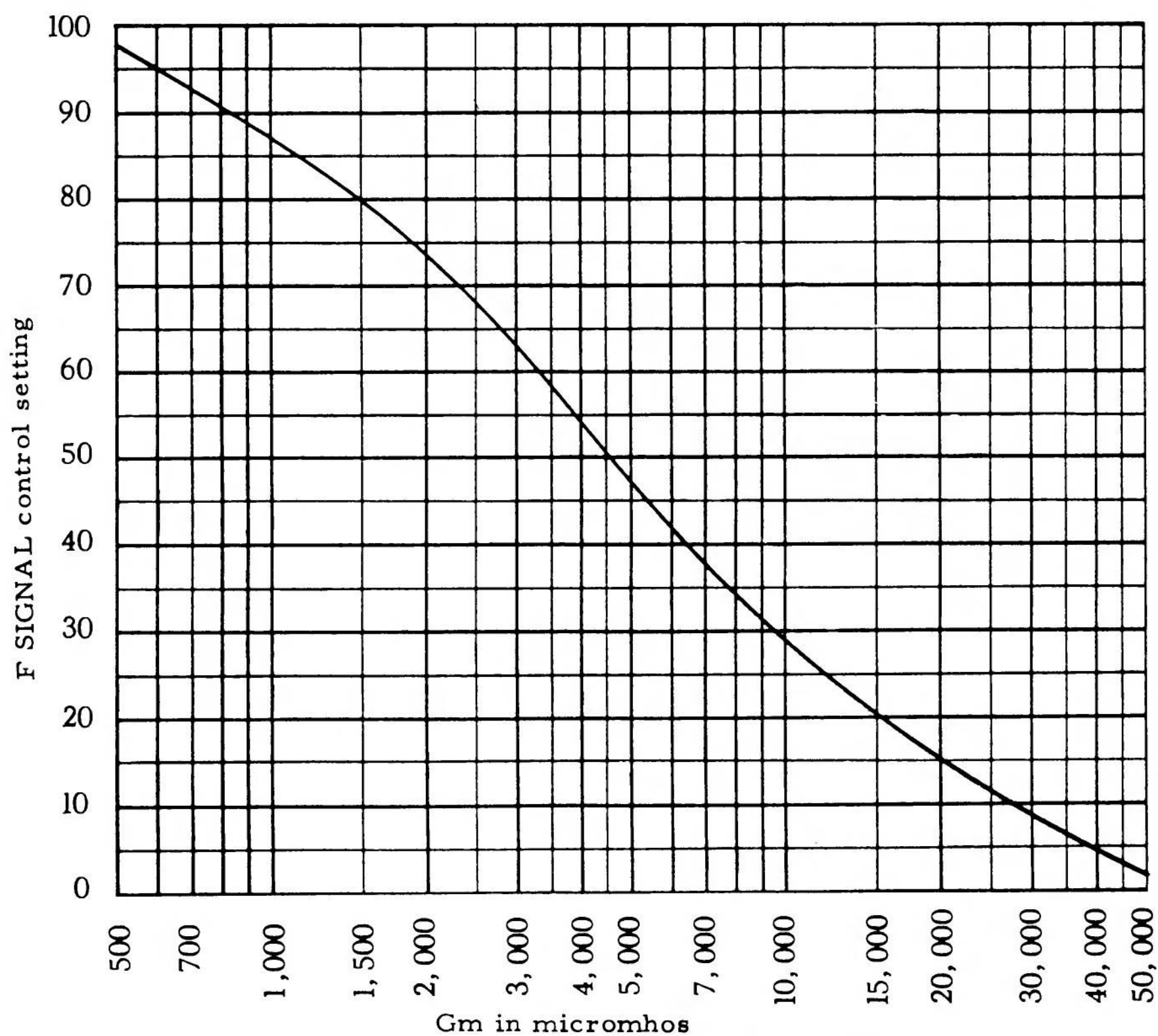
FIGURE 7, MU140 CONVERSION CHART
