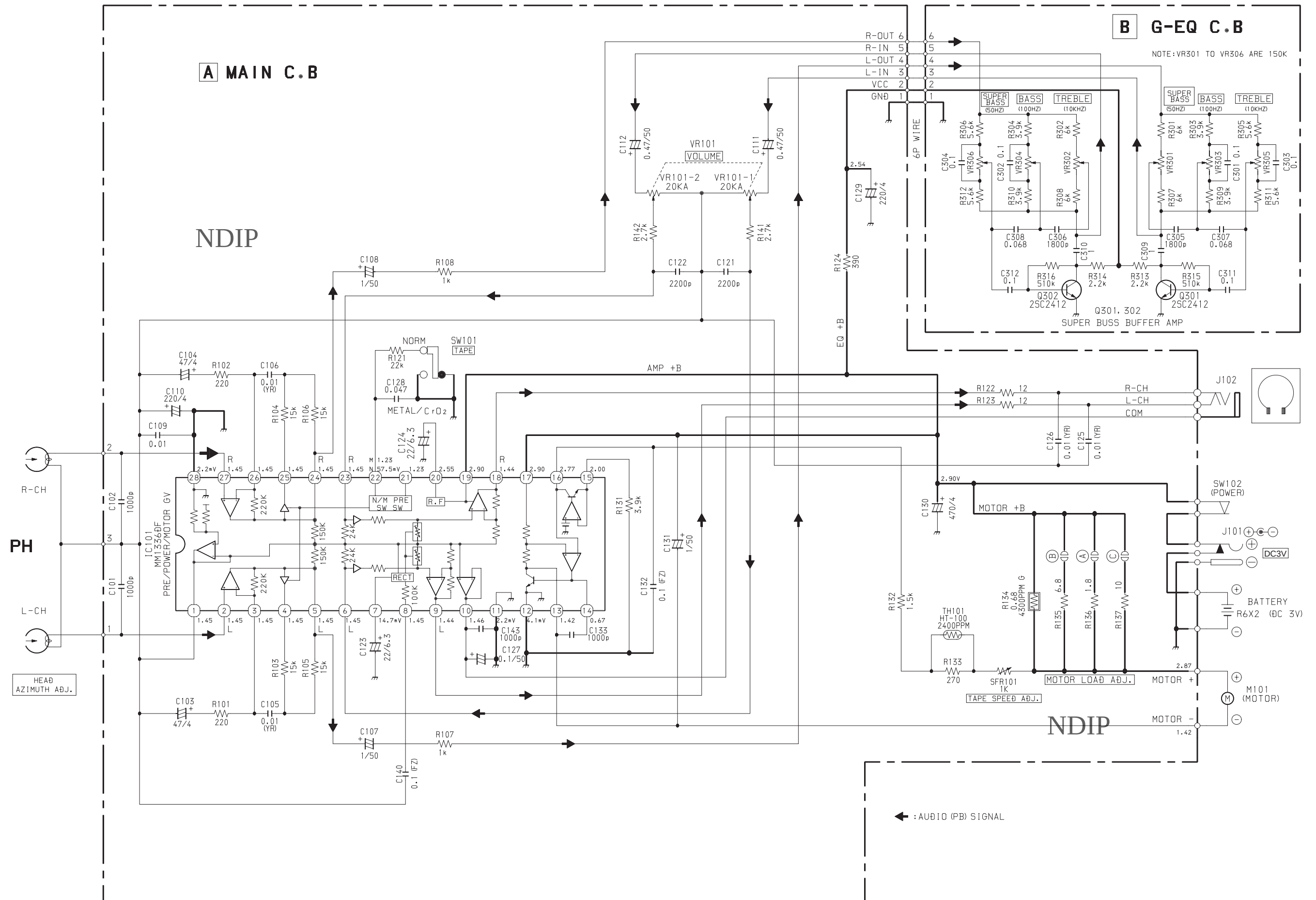
SCHEMATIC DIAGRAM-1
