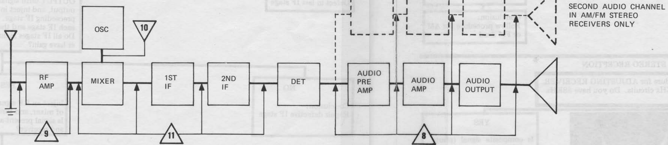
Fig. 54B Block Diagram AM Receiver
