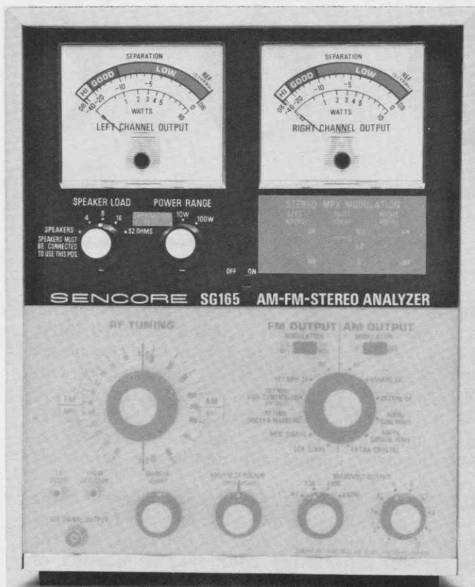
Fig. 11 Output Meters for Power Output Test
