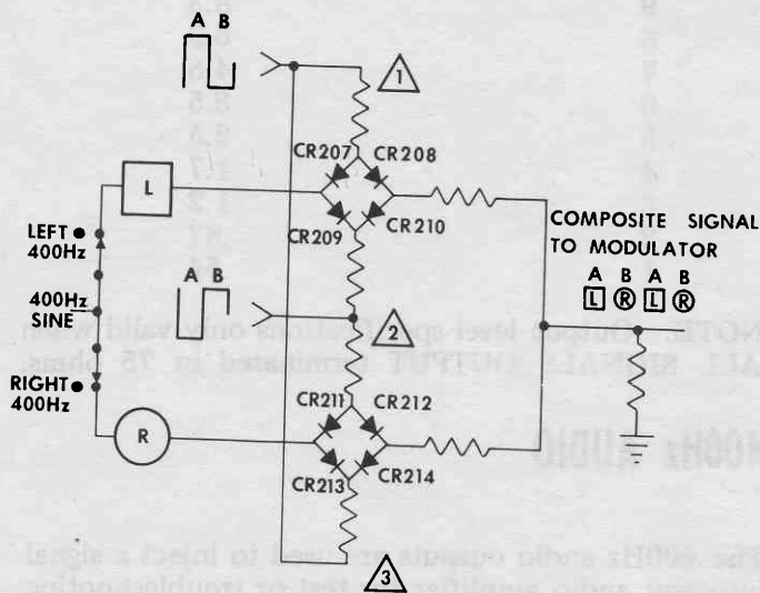
Fig. 24 How the SG165 Generates a Stereo Signal
