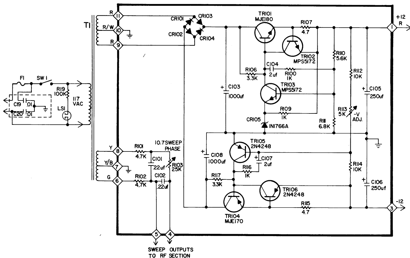
Fig. 69 Power Supply
