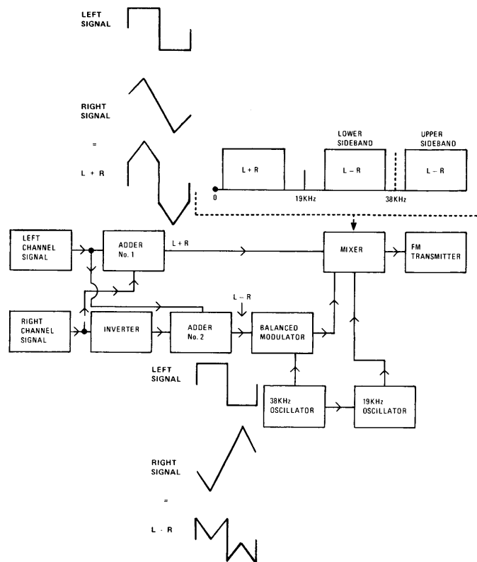
Fig. 26 Block Diagram of FM Stereo Transmitter
