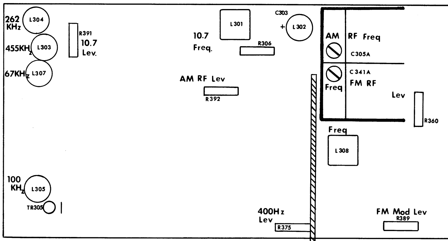
Fig. 55 SG165 Output Calibration Adjustments
