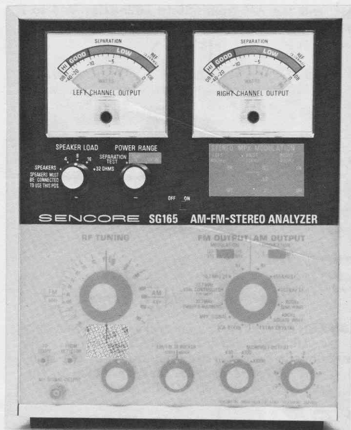
Fig. 10 Output Meters for Separation Test
