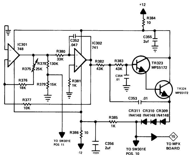
Fig. 62 Audio Oscillator
