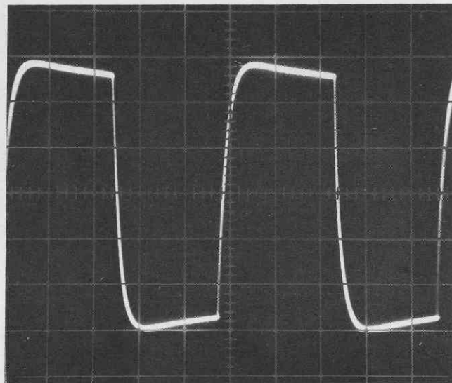
Fig. 42 Auxiliary Input, Treble Control Adjusted to Minimum
