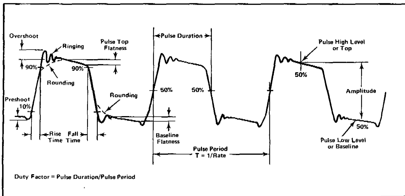
Fig. 1-6. Pulse characteristics.
