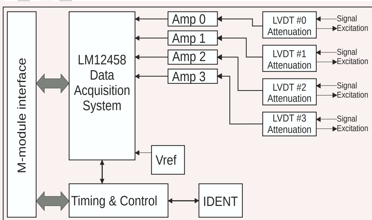
Block diagram
