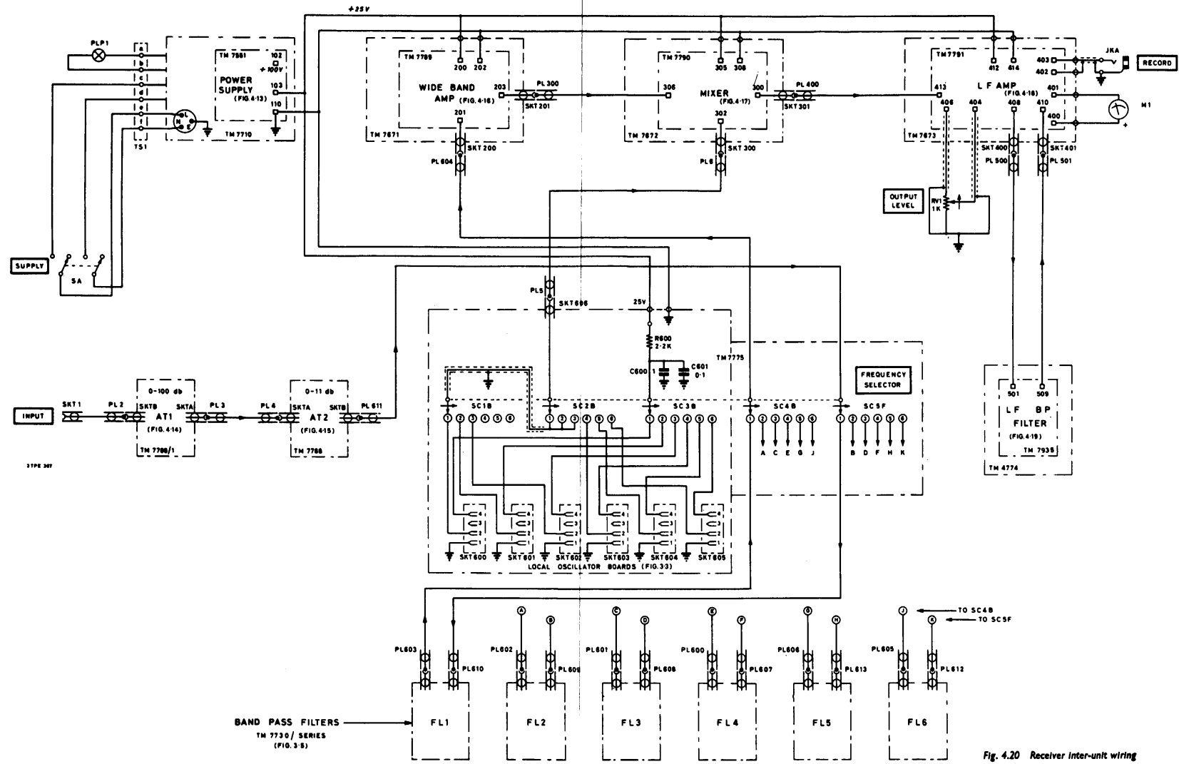
Fig. 4.20 Receiver inter-unit wiring
