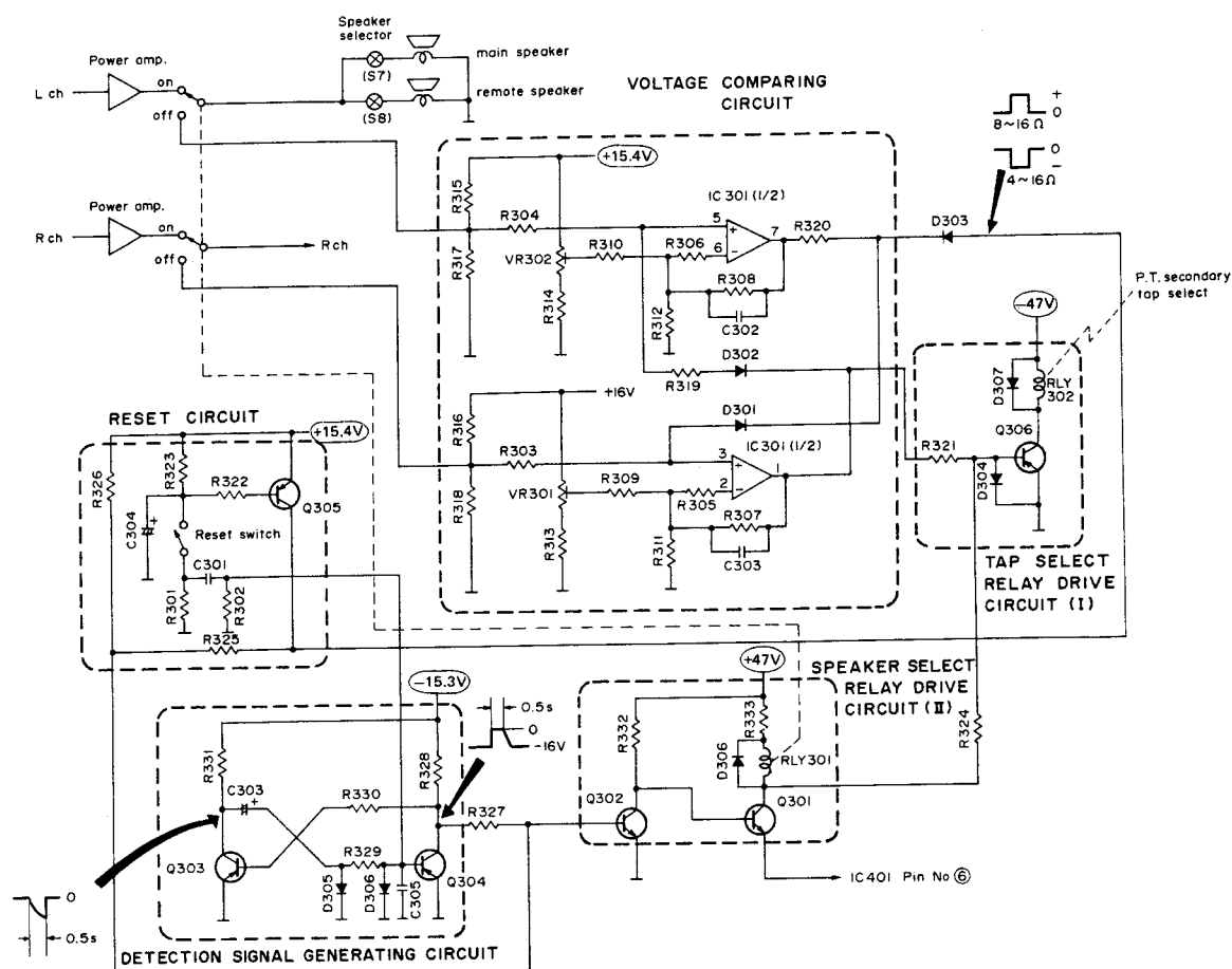
(Speaker impedance detection circuit)
